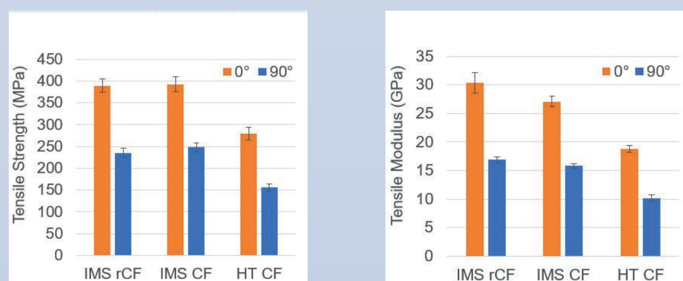
Figure 2: Tensile test results for the laminates (FVC: 25 %) made of carded nonwovens (area weight for single nonwoven layer 300 g/m 2 , fibre length 90 mm)
